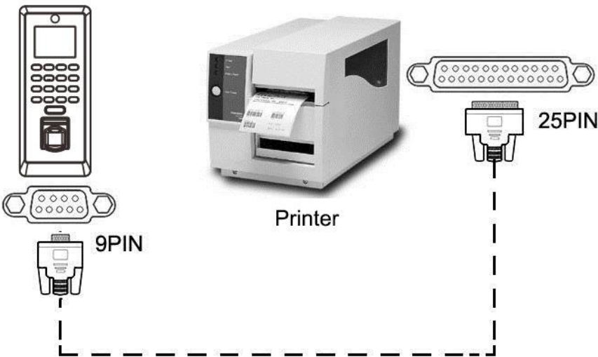
[Connection Diagram]
